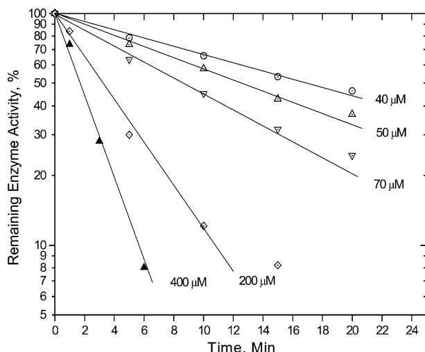
Figure 1. Time dependent inactivation of BPAO by various concentrations of 1,4-diamino-2-butyne ( 4 ).
