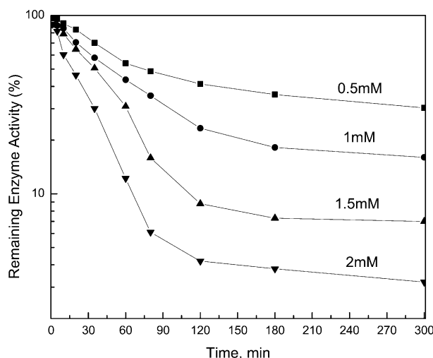
Figure 3. Time dependent inactivation of BPAO by various concentrations of 8 .
