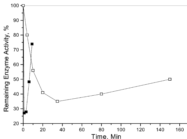
Figure 4. Effect of incubation time on inactivation of BPAO by cis -1,4-diamino-2-butene ( 7 , ■) and N -acetyl-1,4-diamino-2-butyne ( 14 , □).
