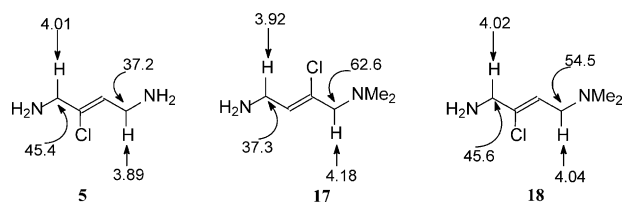
Chart 2. Chemical shift correlation of compounds 5 , 17 , and 18 .
