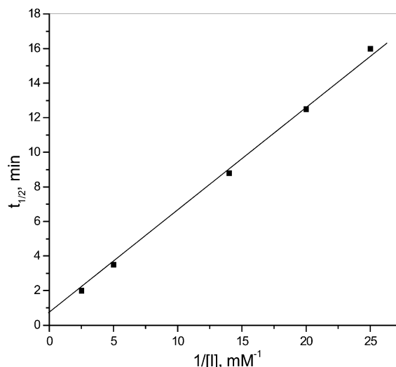
Figure 2. Kitz and Wilson plot for inactivation of BPAO by 4 .
