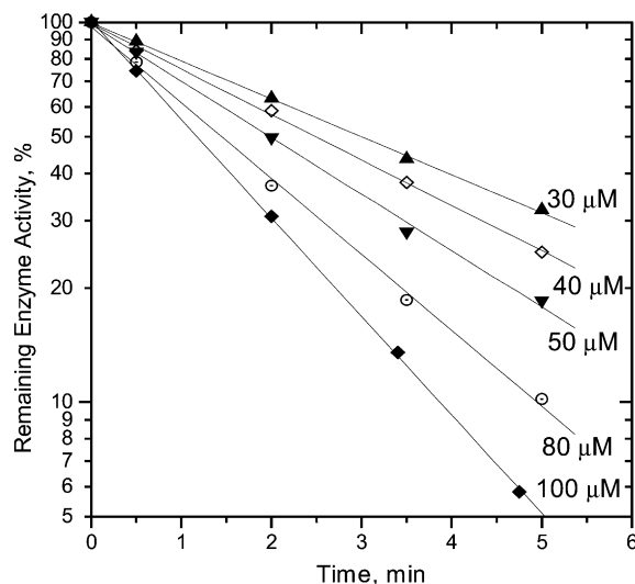
Figure 5. Effect of incubation time on inactivation of BPAO by various concentrations of 5 .
