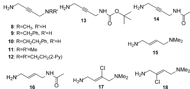
Chart 1. The compounds prepared for evaluation of inhibition of bovine plasma amine oxidase.
