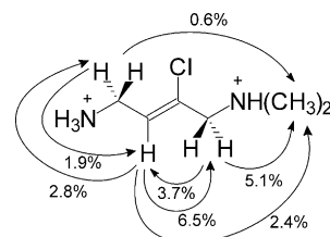
Chart 3. Nuclear Overhauser effect enhancements for compound 17 in CD 3 OD.
